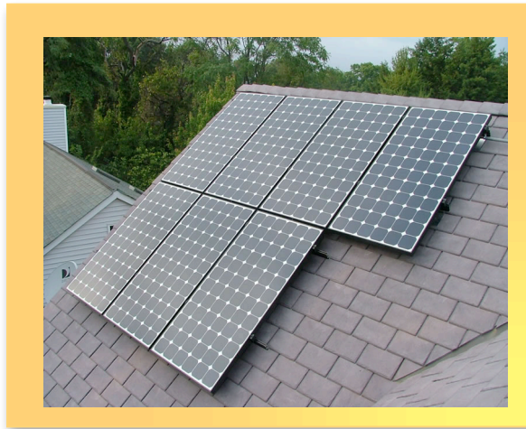
Ward 7 resident Dr. Daanen Strachan’s 3 kW residential solar unit.
